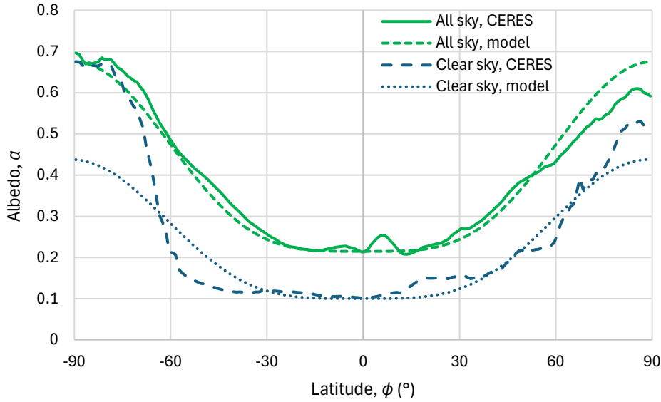
Figure 7.7 Zonal variation of albedo, averaged for each latitude for year 2024. The data are for the top of atmosphere (TOA) from satellites and were retrieved from NASA's CERES site for Terra platform (Edition 4.2). The specific product used here is the CERES SSF1deg monthly averaged observed TOA fluxes grid. The data are available online at https://ceres-tool.larc.nasa.gov/order-tool/jsp/SSF1degEd42Selection.jsp .
