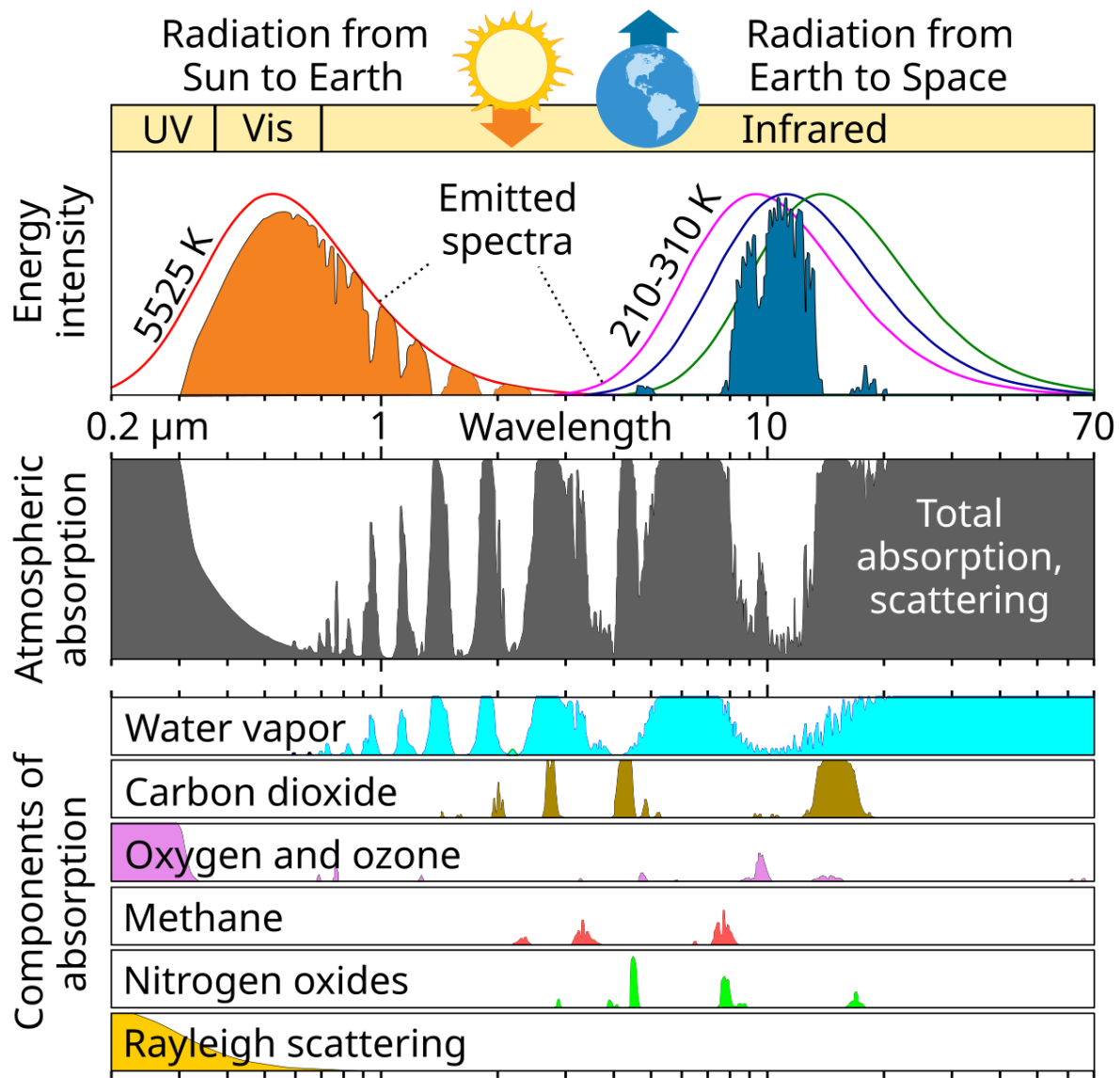
Figure 7.15 Transmission and absorption of SW (solar) and LW (Earth's) radiation through atmosphere, vs. wavelength. The absorption bands of Earth's atmosphere ( middle ) affect both downwelling solar radiation and upgoing LW radiation emitted near the surface ( upper ). The individual absorption spectra of radiatively active gases (plus Rayleigh scattering) are also shown ( lower ) (Source: Wikimedia Commons under a CC license, https://commons.wikimedia.org/wiki/File:Atmospheric_Transmission.svg .)
