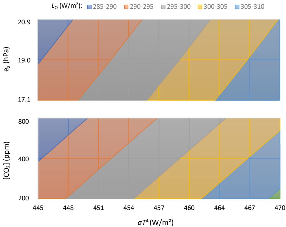
Figure 7.24 As in Figure 7.23 but for the outgoing LW radiation, L_O . (Source: Koutsoyiannis, 2024.)
