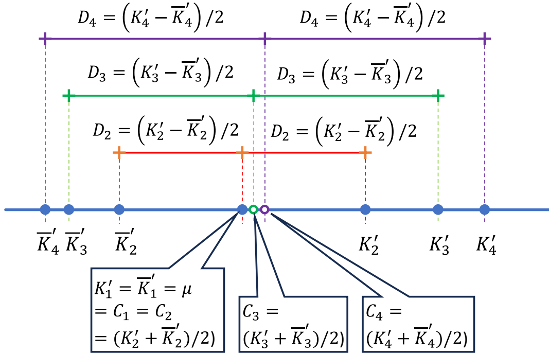
Figure 4.5 Explanatory sketch for the definition of summary statistics based on K-moments. (Source: Koutsoyiannis, 2025a.)
