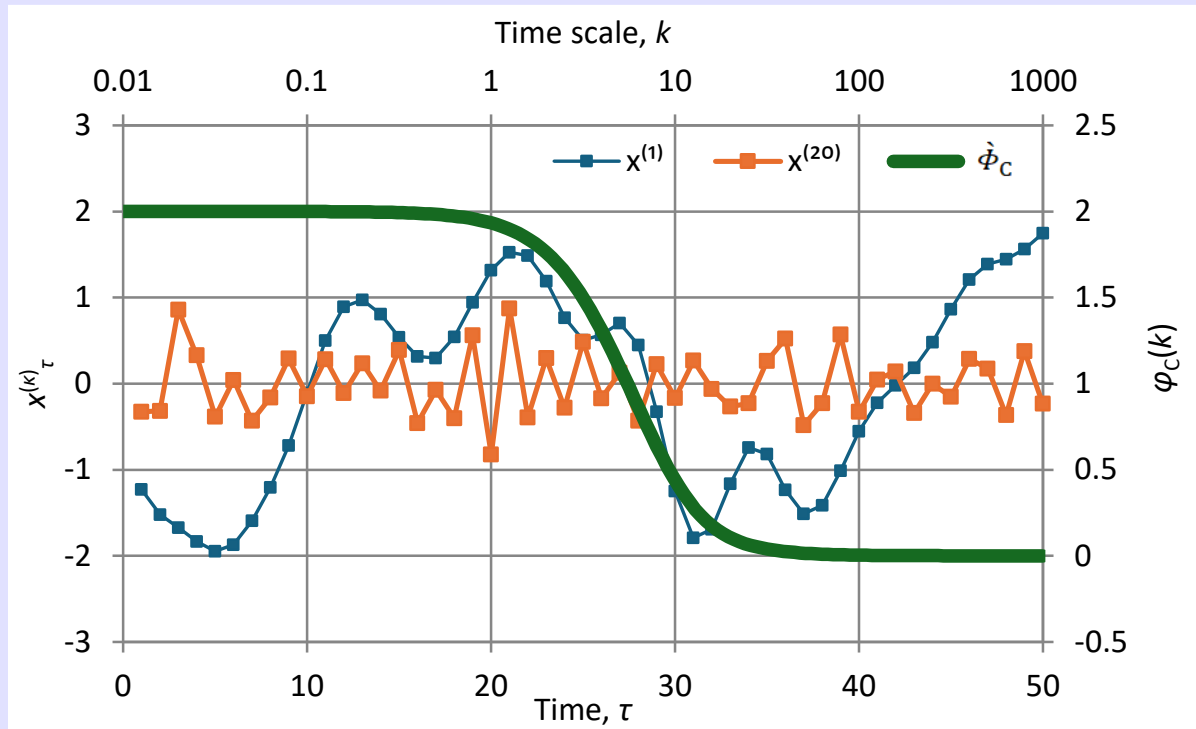
Figure 7.3 The first fifty terms at time scales k = 1 and 20 of time series representing the blackbody radiation process, produced by the exact model, along with the “stamp” of the model (thick line plotted with respect to the right vertical axes) represented by the CEPLT, \phi_c(k) . Notice the similarity to the plot in Figure 3.8(f).
