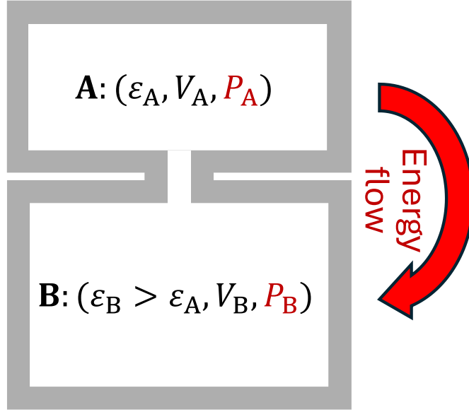
Figure 6.8 Explanation sketch for the non-equilibrium open interaction of two systems in contact, showing the characteristics in each system, where those typeset in black are known and those in red are determined by entropy maximization.
