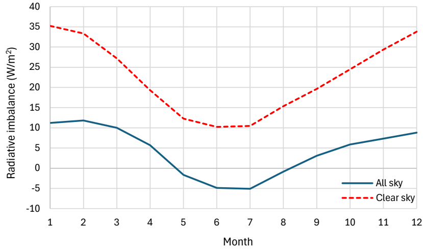
Figure 7.14 Monthly distribution of global average radiative (SW and LW) imbalance at TOA for year 2024 according to CERES satellite data. A positive imbalance means that Earth gains energy. The global annual averages are 4 and 23 W/m 2 for all and clear sky, respectively. Data from NASA's CERES site for Terra platform (Edition 4.2; https://ceres-tool.larc.nasa.gov/ord-tool/jsp/SSF1degEd42Selection.jsp ).
