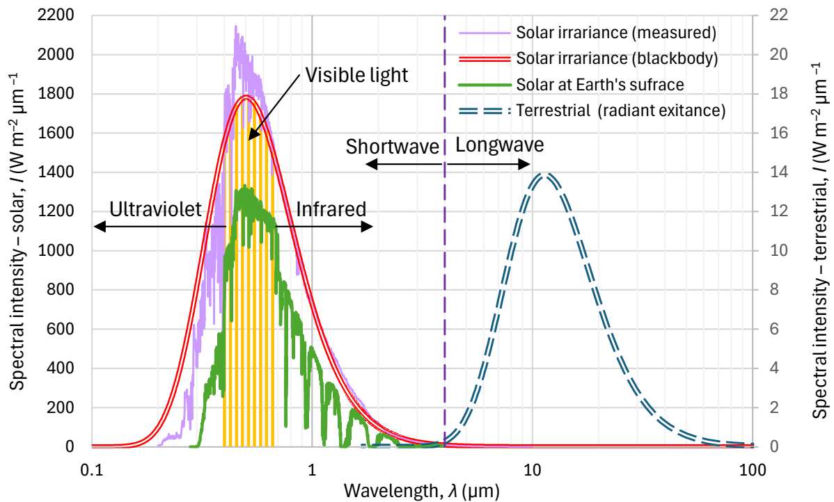
Figure 7.2 Comparison of (a) observed solar irradiance at the top of Earth's atmosphere; (b) the theoretical blackbody radiation intensity of the Sun viewed from Earth (irradiance, I_{\lambda}(\lambda, \theta, d) = \Omega_d B_{\lambda}(\lambda, \theta) for \Omega_d = 6.794 \times 10^{-5} sr as in Figure 7.1); (c) average solar radiation reaching Earth's surface; (d) terrestrial (Earth's) blackbody radiation (spectral radiant exitance, M_{\lambda}(\lambda, \theta) , as in Figure 7.1). For the solar spectrum, the total power (area of each spectrum) is 1361 and 735 W/m 2 at the top of atmosphere and the surface, respectively, which, if reduced to Earth's area (by division by 4), become 340 and 184 W/m 2 , respectively. For the plotted terrestrial spectrum, the total power is 240 W/m 2 . Notice that for the terrestrial radiation the intensities are by two orders of magnitude lower, as in the right vertical axis. Data origin: (i) for the solar irradiance: 2000 ASTM Standard Extraterrestrial Spectrum Reference E-490-00, https://www.nrl.gov/media/docs/libraries/grid/e490_00a_amo.xls (ii) for the solar spectrum at Earth's surface, ASTM G173-03 Reference Spectra Derived from SMARTS v. 2.9.2 available from the NREL Solar Spectra Page, https://www.nrel.gov/media/docs/libraries/grid/astmg173.xls (Global tilt data, after adaptation as described in text).
