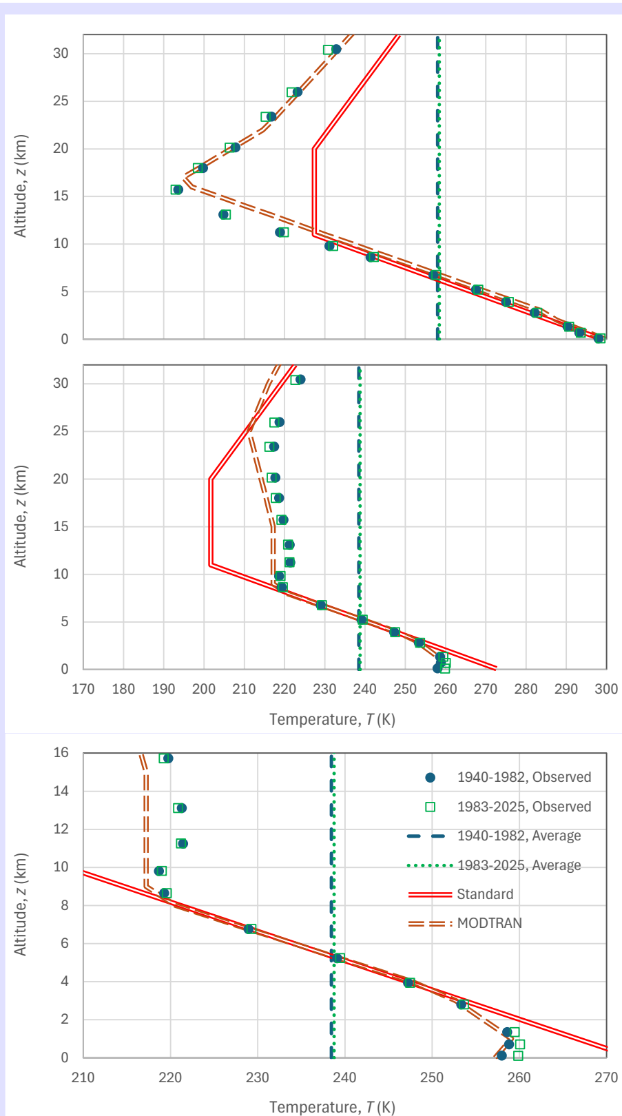
Figure 6.21 ERA5 temperature (marked as “observed”) vs. ERA5 geopotential height, as in Figure 6.20, but averaged over the entire year for two periods of equal length of 43 years as indicated in the figure legend: (upper) for the tropical zone extending \pm 7.5^\circ around the equator (middle) the polar zone of width 7.5^\circ south of the north pole, and (lower) zoom in of the middle panel. For the polar profile (middle and lower) the shift of the standard profile was chosen so as to better fit the observed profile, rather than to match the surface temperature. For the same reason the subarctic winter profile of MODTRAN is plotted in the middle and lower panels, as it better fits the troposphere data.
