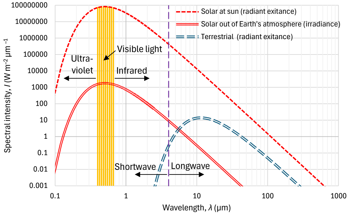
Figure 7.1 Blackbody radiation intensity for the Sun's surface (spectral radiant exitance, M_\lambda(\lambda, \theta) , for T = 5772 K, \theta = T/k_B ) and Sun viewed from Earth (irradiance, I_\lambda(\lambda, \theta, d) = \Omega_d B_\lambda(\lambda, \theta) for \Omega_d = 6.794 \times 10^{-5} sr), in comparison to terrestrial (Earth's) blackbody radiation (spectral radiant exitance, M_\lambda(\lambda, \theta) , for T = 255 K, \theta = T/k_B ). Classification of radiation based on wavelength is also shown, with visible light defined between 0.4 and 0.7 \mu\text{m} and the boundary between solar (shortwave, SW) and terrestrial (longwave, LW) radiation defined at a wavelength of 4 \mu\text{m} . The wavelengths at which the intensity is maximized (equation (7.24)) are 0.502 \mu\text{m} and 11.36 \mu\text{m} for solar and terrestrial radiation, respectively. The temperature T = 255 K is the mean temperature of the Earth's atmosphere (see section 7.4 for justification).
