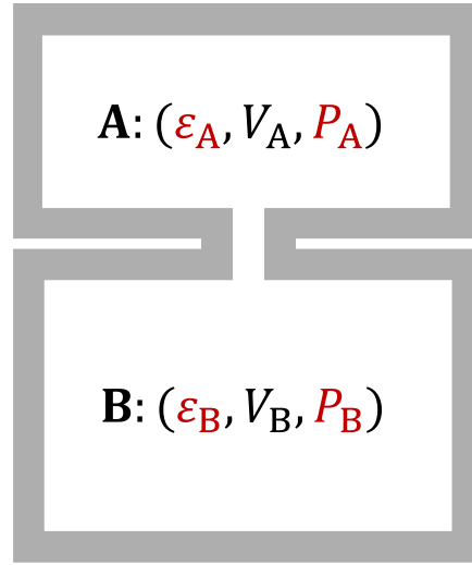
Figure 6.5 Explanation sketch for the open interaction of two systems in contact, showing the characteristics in each system, where those typeset in black are known and those in red are determined by entropy maximization.
