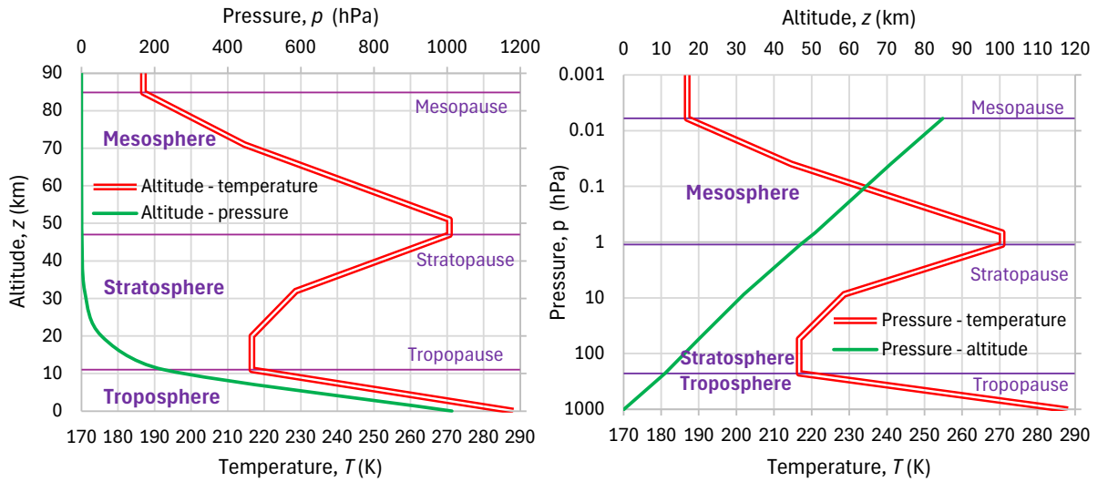
Figure 6.18 Vertical profiles of the ICAO (1993) standard atmosphere: (left) temperature and pressure as functions of altitude; (right) temperature and altitude as functions of pressure. (Source: Koutsoyiannis and Tsakalias, 2025.)
