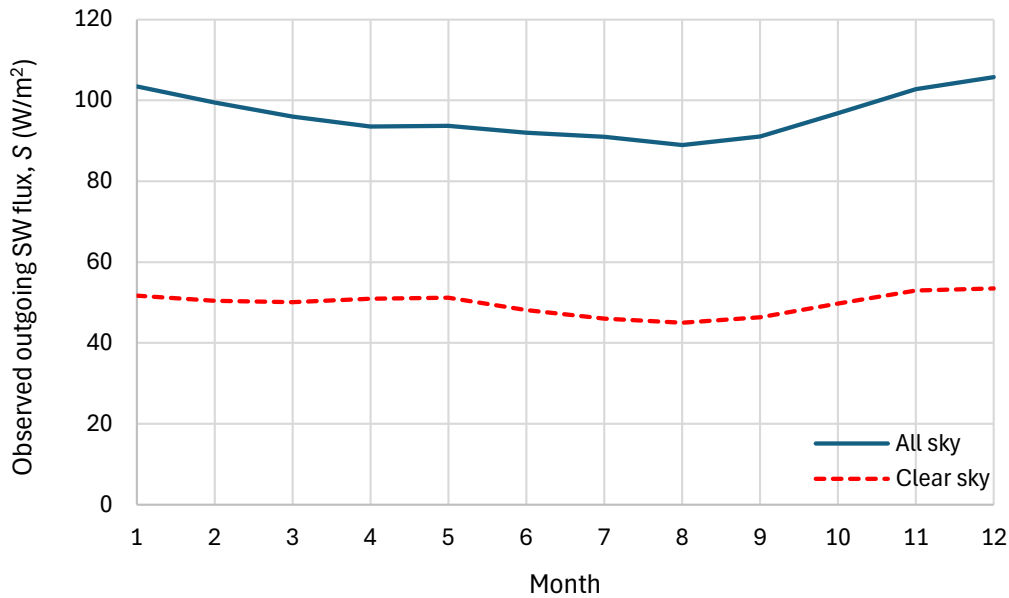
Figure 7.10 Monthly variation of outgoing solar radiation flux for 2024. The annual average is 96.2 and 49.7 W/m 2 for all sky and clear sky, respectively. Data from NASA’s CERES site for Terra platform (Edition 4.2; https://ceres-tool.larc.nasa.gov/ord-tool/jsp/SSF1degEd42Selection.jsp ).
