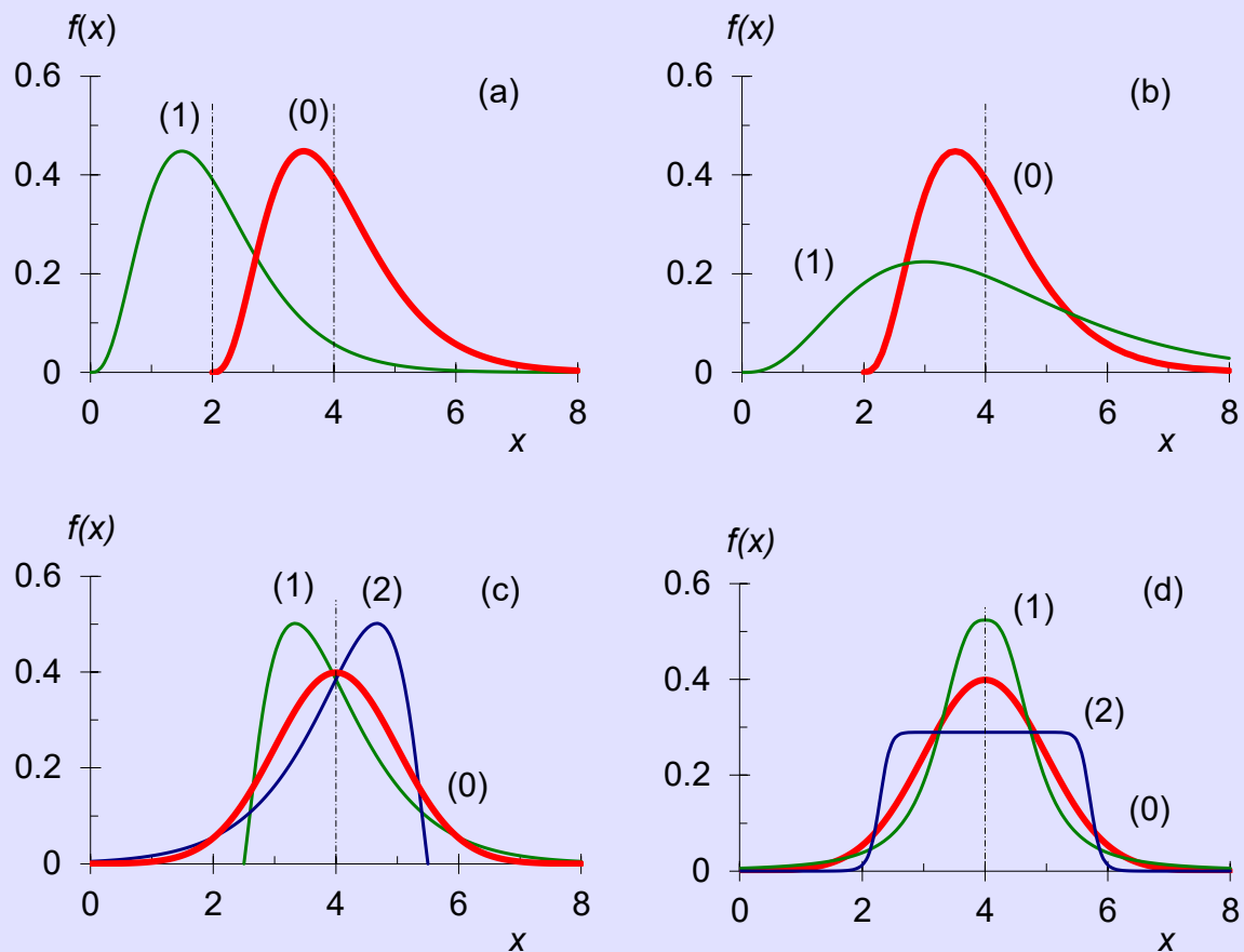
Figure 2.4 Graphical illustration of the geometrical interpretation of moments of a stochastic variable: (a) Effect of the mean. Curves (0) and (1) have means 4 and 2, respectively, whereas they both have standard deviation 1, coefficient of skewness 1 and coefficient of kurtosis 4.5. (b) Effect of the standard deviation. Curves (0) and (1) have standard deviation 1 and 2 respectively, whereas they both have mean 4, coefficient of skewness 1 and coefficient of kurtosis 4.5. (c) Effect of the coefficient of skewness. Curves (0), (1) and (2) have coefficients of skewness 0, +1.33 and -1.33, respectively, but they all have mean 4 and standard deviation 1; their coefficients of kurtosis are 3, 5.67 and 5.67, respectively. (d) Effect of the coefficient of kurtosis. Curves (0), (1) and (2) have coefficients of kurtosis 3, 5 and 2, respectively, whereas they all have mean 4, standard deviation 1 and coefficient of skewness 0.
