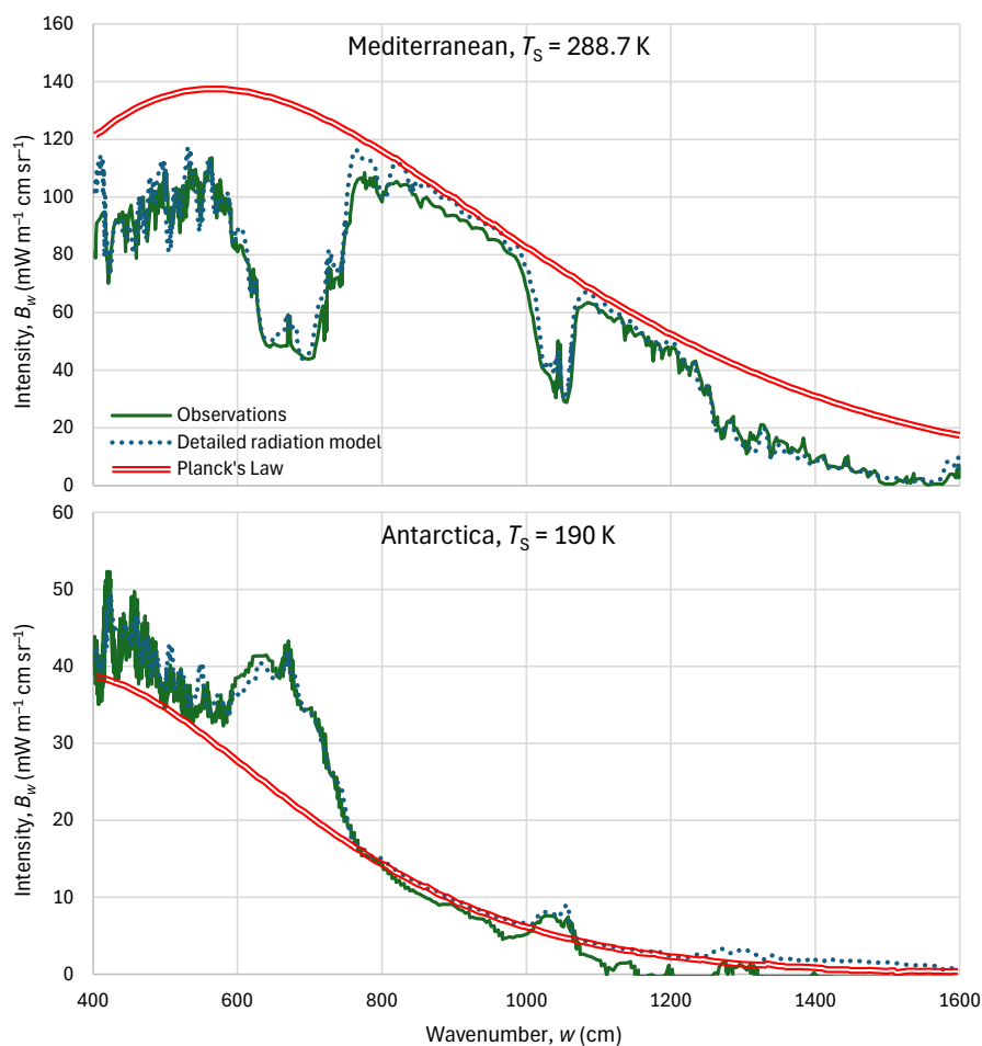
Figure 7.21 Vertical intensities at the TOA observed with a Michaelson interferometer in a satellite (Hanel and Conrath, 1970), and modelled with radiation transfer theory for the Mediterranean and Antarctica. (Reproduction with adaptation of part of Figure 9 in van Wijngaarden and Happer, 2025.)
