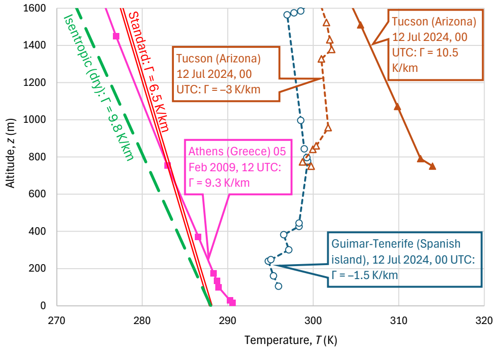
Figure 6.12 Lower troposphere profiles as observed by radiosondes at the indicated sites and dates. The slopes noted are calculated by linear regression on the points shown on the graph (not the entire range covered by radiosonde data). The profiles with continuous and dashed lines correspond to daytime and nighttime, respectively. The standard atmospheric profile and an isotropic profile are also shown. (Data retrieved from the University of Wyoming Atmospheric Science Radiosonde Archive, https://weather.uwyo.edu/upperair/sounding.shtml ).
