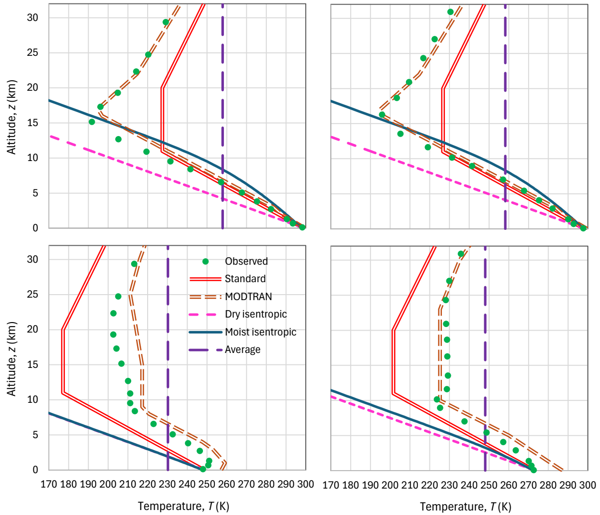
Figure 6.20 ERA5 temperature (marked as “observed”) vs. ERA5 geopotential height, spatially integrated over ocean grid points at ( upper row ) a tropical zone extending \pm 7.5^\circ around the equator and ( lower row ) a polar zone of width 7.5^\circ south of the north pole, in comparison to (a) the profile of the standard atmosphere (shifted to match the temperature at z = 0 ), (b) the closest MODTRAN profile (namely the tropical profile for the upper row, and the subarctic winter and summer profiles for the left and right panels of the lower row, respectively), (c, d) the dry and moist isentropic profiles, and (e) the isothermal profile with the average temperature. The temperature plots are for mean monthly scale and specifically for the months of ( left column ) February and ( right column ) August.
