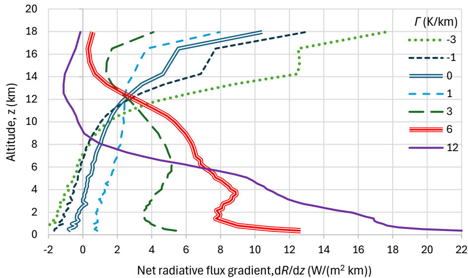
Figure 7.20 Vertical distribution of net radiation flux gradient for the RRTM runs of Figure 7.17 assuring the energy balance, vs. lapse rate. For better presentation smoothing of the original values was performed by taking moving averages over five adjacent values.
