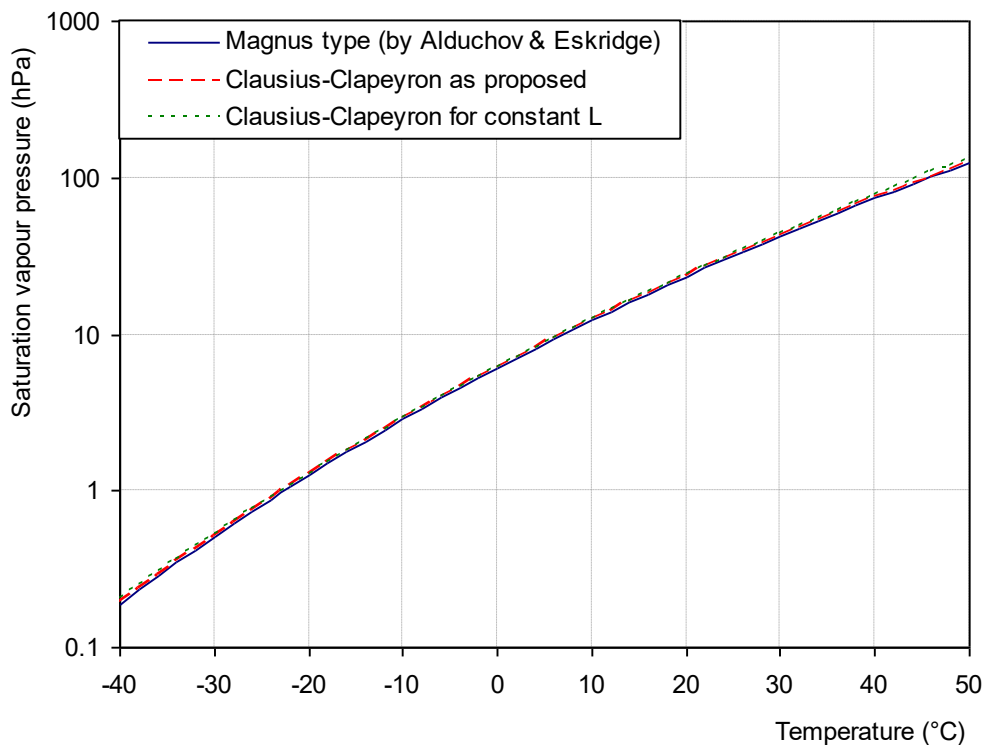
Figure 6.15 Comparison of the saturation water vapour pressure obtained by the consistent equation (6.200) as well as by the standard but inconsistent equation (6.201). In addition, an empirical equation, e/\text{hPa} = 6.1094 \exp((17.625 T/^\circ\text{C})/(243.04 + T/^\circ\text{C})) from Alduchov & Eskridge (1996) is also compared. (Source: Koutsoyiannis, 2012.)
