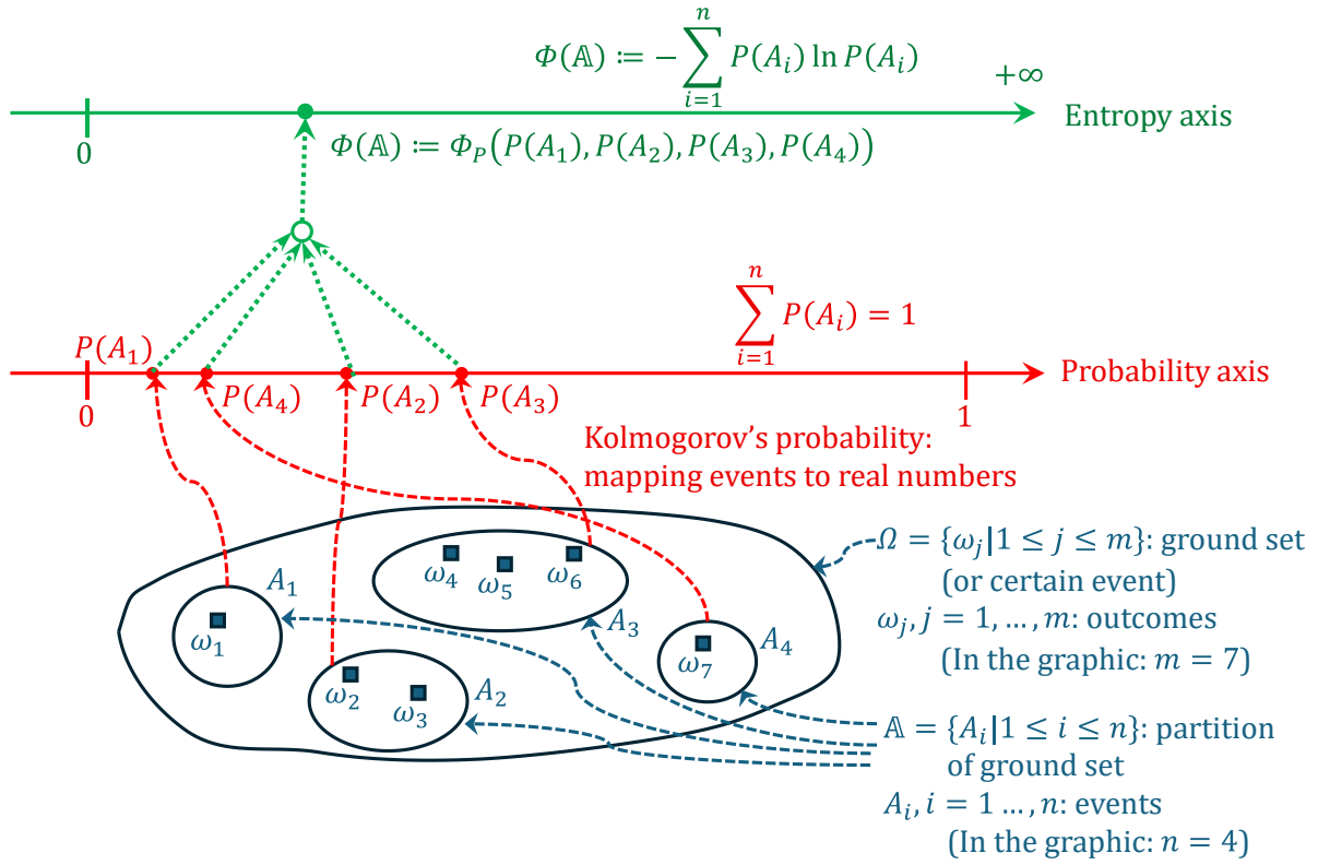
Figure 2.1 Schematic for the basic concepts required for entropy definition: ground set, outcomes, events, partition, and probability and entropy as functions.
