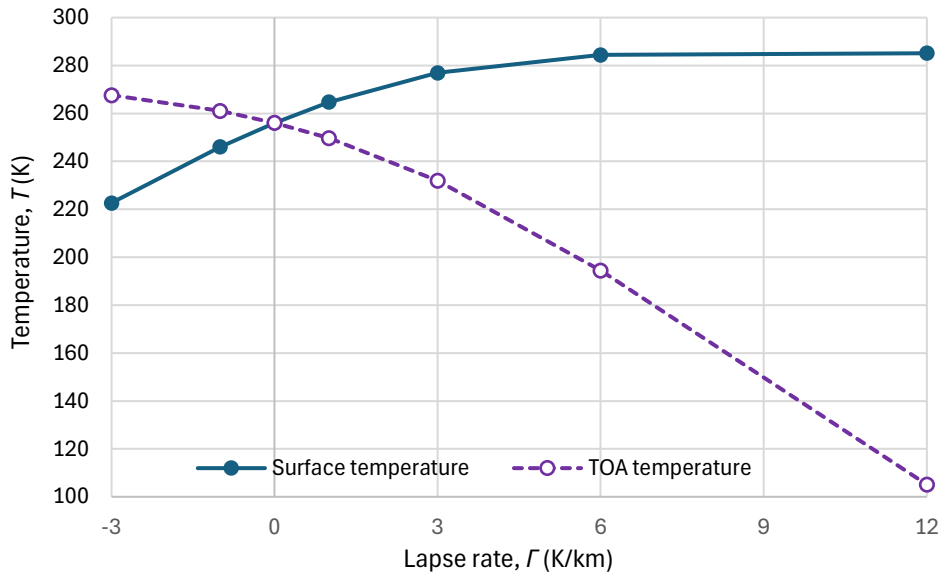
Figure 7.17 Surface and TOA temperatures leading to energy balance vs. lapse rate, as calculated from RRTM runs using default parameters (without clouds).
