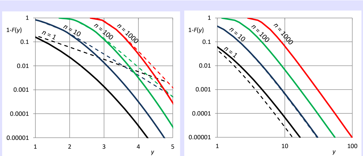
Figure 2.10 Approximation of the true distribution of the maximum of n independent identically distributed variables (continuous lines) by the limiting extreme value distribution (dashed lines). (left) The parent distribution is the standard normal, N(0,1) , and the approximating distribution is the EV1. (right) The parent distribution is the Pareto, F(x) = 1 - (1 + x)^{-1/\xi} , with \xi = 0.25 and the approximating distribution is the EV2 with the same \xi .
