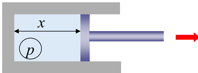
Figure 6.3 Explanation sketch showing a piston moving under the influence of the inside gas pressure p (the external pressure is taken as zero).
