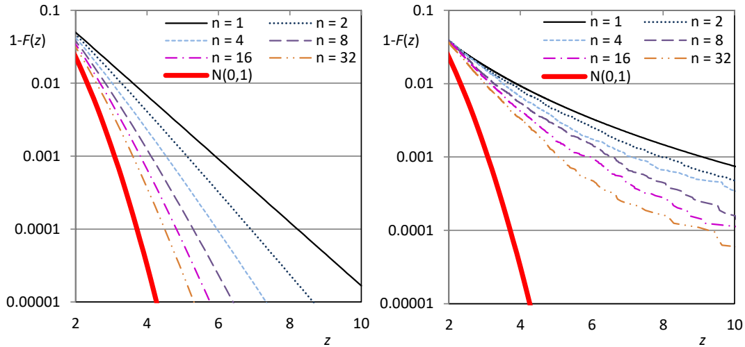
Figure 2.9 Convergence of the sum of independent identically distributed stochastic variables to the normal distribution (thick line) with focus on the upper tail. The thin continuous lines represent the exceedance probability of the constituent variables \underline{x}_i , which have mean 0 and standard deviation 1. In the left panel the distribution is exponential with density f(x) = e^{-x-1}, x > -1 as in the right panel of Figure 2.8) and in the right panel Pareto with upper-tail index 1/4 and exceedance probability \bar{F}(x) = \left(4/3 + \frac{x\sqrt{2}}{3}\right)^{-4}, x \geq -1/\sqrt{2} (the parameters are chosen so that the mean is 0 and standard deviation 1). The dotted lines represent the exceedance probability of the sums \underline{z}_n := (\underline{x}_1 + \dots + \underline{x}_n)/\sqrt{n} for the values of n indicated in the legend. The left graph was produced from equations (2.53) and (2.138), and the right graph by a numerical (Monte Carlo) method (as analytical integration is impossible beyond n = 2 ), and this is the reason for the curly shape of the curves.
