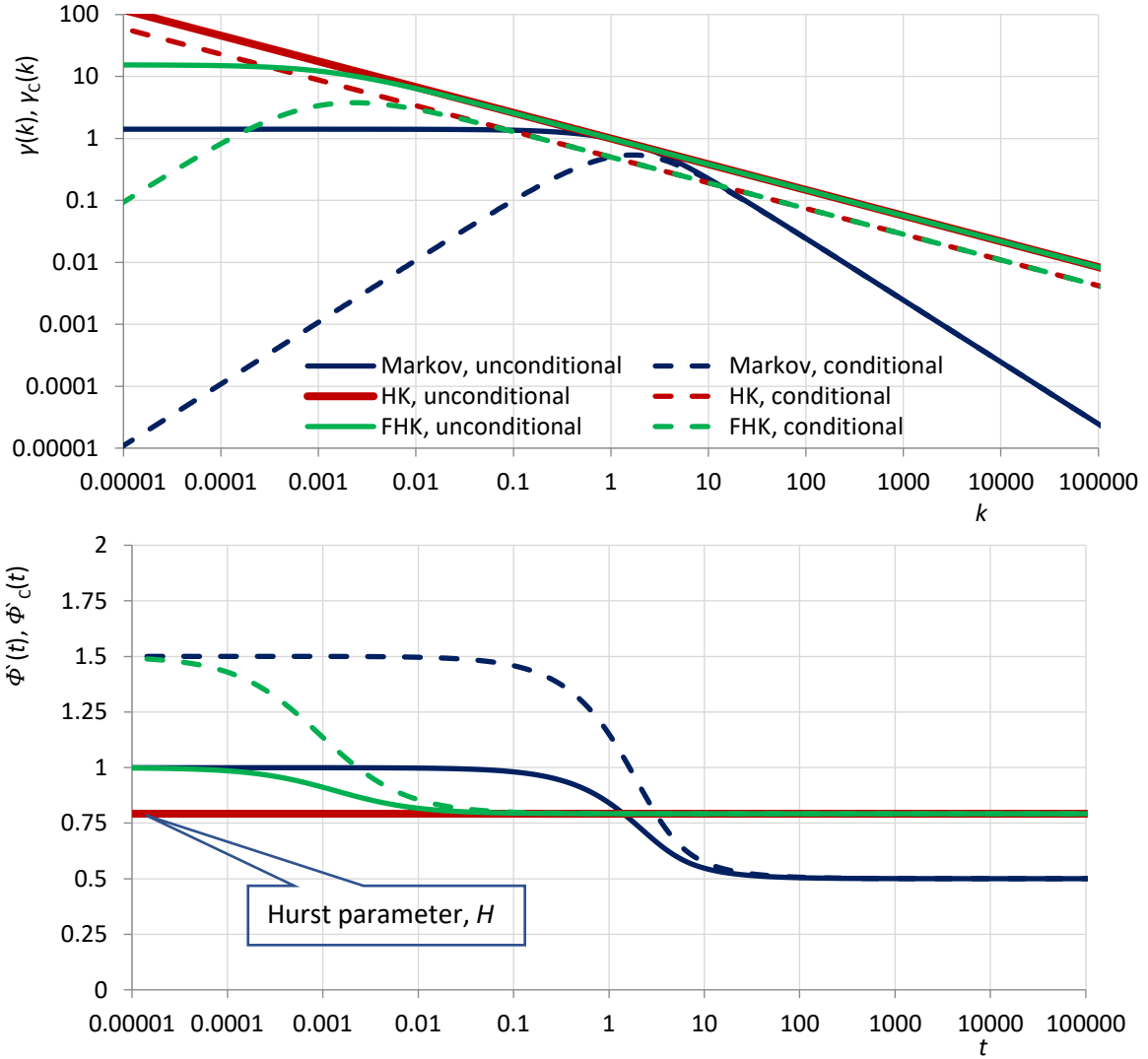
Figure 3.7 (upper) Climacograms and (lower) EPLT ( \dot{\Phi}(t) ) and CEPLT ( \dot{\Phi}_c(t) ) of the three indicated example processes for neutral smoothness ( M = 0.5 ). At time scale D = 1 all three processes have the same variance \gamma(1) = 1 and the same autocovariance for lag 1, c_1^{(1)} = 0.5 . Their parameters are: for the linear Markov process a = 0.8686 , \lambda = 1.4176 ; for the HK process a = 0.0013539 , \lambda = 15.5032 , H = 0.7925 (equivalently, a = \lambda = 1 but the former parameter set was preferred in order to be comparable to the FHK); for the FHK process a = 0.0013539 , \lambda = 15.5093 , M = 0.5 , H = 0.7925 . In the lower graph conditional and unconditional HK coincide (adapted from Koutsoyiannis, 2016).
