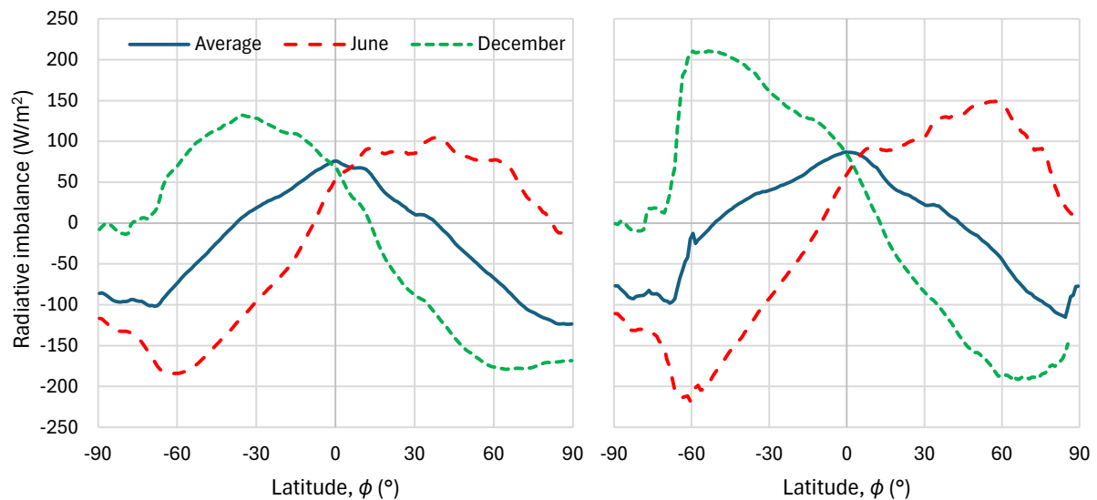
Figure 7.13 Zonal distribution of annual average radiative (SW and LW) imbalance at TOA (from monthly data of year 2024) according to CERES satellite data for (left) all sky and (right) clear sky. A positive imbalance means that Earth gains energy. The global annual averages are 4 and 23 W/m 2 for all and clear sky, respectively. Data from NASA's CERES site for Terra platform (Edition 4.2; https://ceres-tool.larc.nasa.gov/ord-tool/jsp/SSF1degEd42Selection.jsp ).
