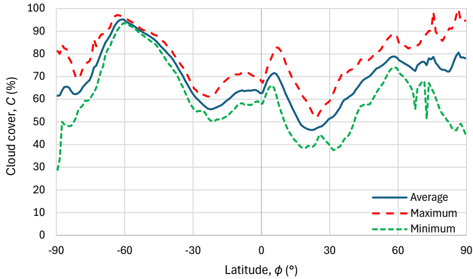
Figure 7.11 Zonal distribution of annual average daytime cloud area cover (from monthly data of year 2024). The global annual average is 66%. Data from NASA's CERES site for Terra platform (Edition 4.2; https://ceres-tool.larc.nasa.gov/ord-tool/jsp/SSF1degEd42Selection.jsp ).
