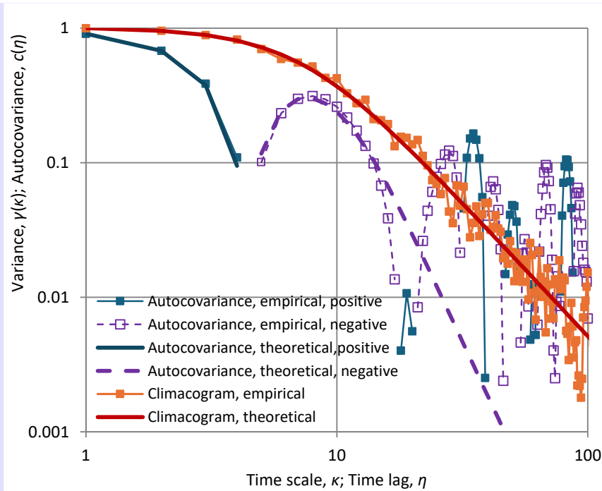
Figure 7.4 Empirical (estimated by the generated time series) and theoretical climacogram and autocovariance function (determined from the exact model). Notice that the autocovariance is negative beyond lag 4 and the negative part is plotted separately in the double logarithmic graph, after sign change. Beyond lag 20 the autocovariance function is too noisy and provides no information.
