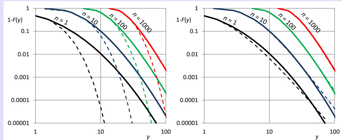
Figure 2.11 Approximation of the true distribution of the maximum of n independent variables with lognormal distribution LN(0,1) (continuous lines) by the limiting extreme value distribution (dashed lines), which is (left) EV1 and (right) EV2 with \xi = 0.3/n^{0.07} , which was found after a numerical investigation and fitting a power function of n by minimizing the fitting error.
