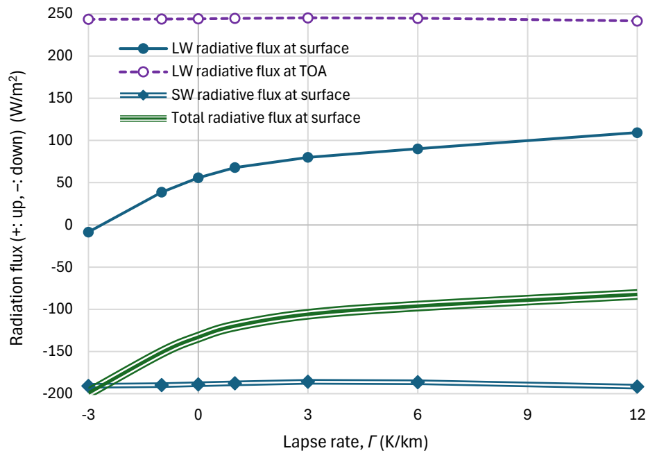
Figure 7.18 Surface and TOA radiation flux for the indicated levels for the RRTM runs of Figure 7.17 assuring the energy balance, vs. lapse rate.
