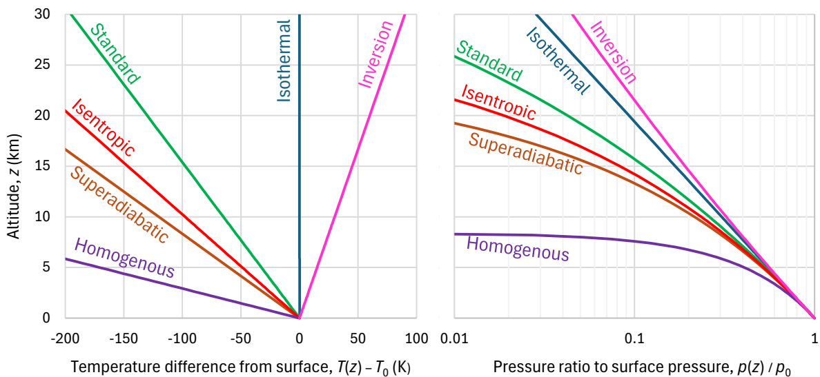
Figure 6.11 (left) Temperature profile, expressed as the difference from the surface temperature, and (right) pressure profile, expressed as the ratio to the surface pressure, for the entropy profiles shown in Figure 6.10 and for surface temperatures T_0 equal to 288 K.
