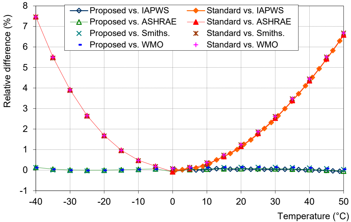
Figure 6.16 Comparison of relative differences of the saturation water vapour pressure obtained by the consistent equation (6.200) as well as by the inconsistent equation (6.201), with observed data. Four reference data sets are used, which are given in tabulated form from different origins: (a) the International Association for the Properties of Water and Steam(IAPWS), (b) the Smithsonian Meteorological Tables (Smiths.), (c) the World Meteorological Organization (WMO) meteorological tables, and (d) the American Society of Heating, Refrigerating and Air-conditioning Engineers (ASHRAE). (Source: Koutsoyiannis, 2012.)
