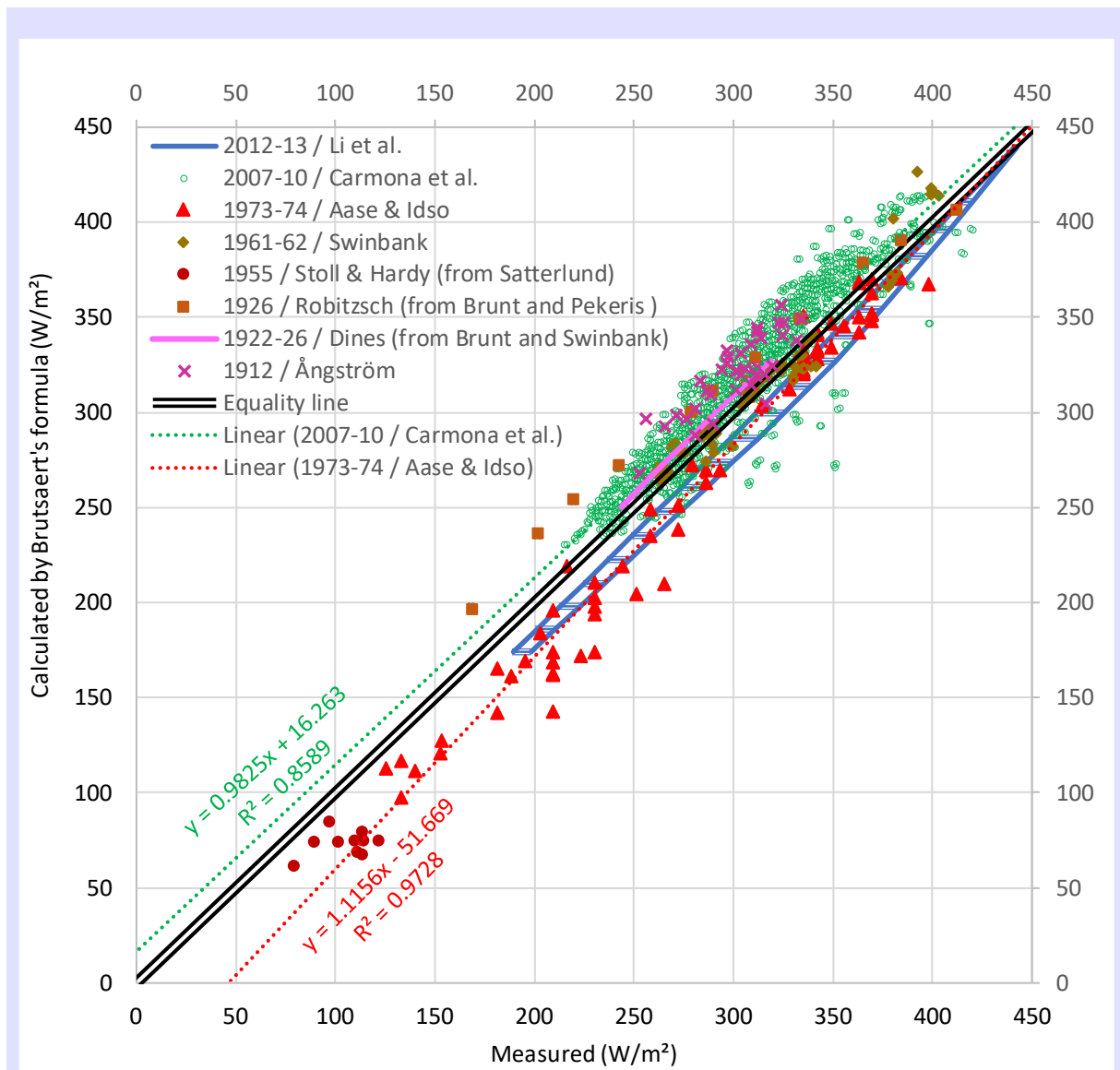
Figure 7.16 Plot of downward radiation of the atmosphere L_A calculated by the Brutsaert's formula with its original parameters (equation (7.70)), vs. measured L_A in eight data sets distributed across a century. The points correspond to individual measurements, while the lines correspond to reconstructions by envelopes, as described in the study by Koutsoyiannis and Vournas (2024). For the two data sets with the largest number of points (1973-74, 2007-10), the linear regression lines are also shown in the figure, along with their equations. (Source: Koutsoyiannis and Vournas, 2024, where the origin of each data set is explained.)
