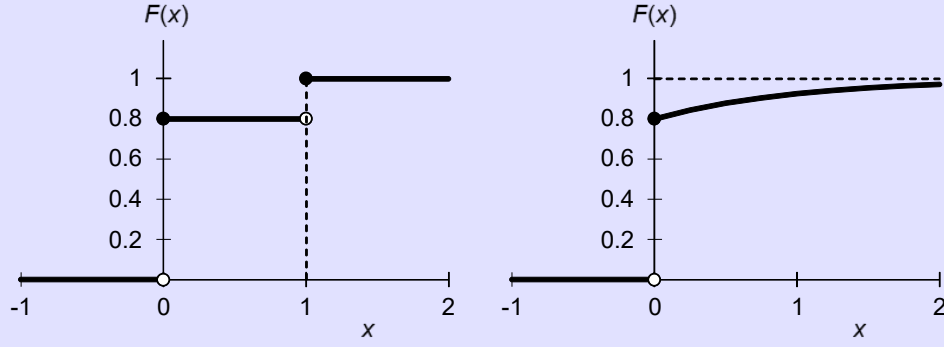
Figure 2.3 Distribution function of a stochastic variable representing events related to rainfall on a given day in a certain area and at a specific time of the year: (left) the dry or wet state; (right) the rainfall depth.
