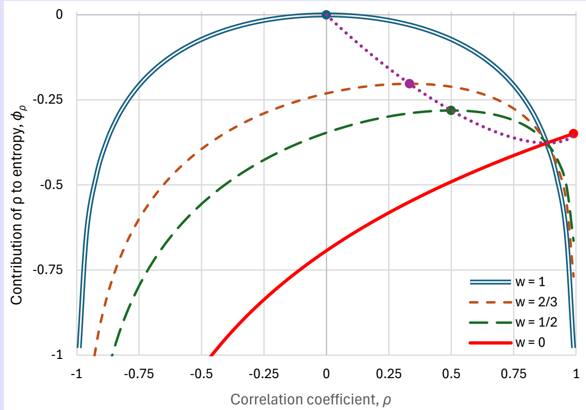
Figure 6.22 Contribution to the entropy, \varphi_\rho , of the correlation between to particles, \rho , as a function of \rho and the weight w given to the entropy of a single particle. The dots represent the points in which \varphi_\rho is maximized and the dotted line, depicting \varphi_\rho^{\max} , connects these points.
