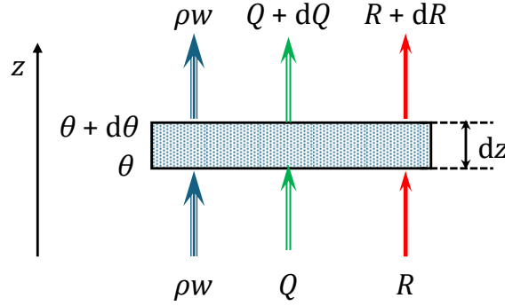
Figure 6.24 Schematic of an atmospheric layer (control volume) of area A and height dz at (natural) temperature \theta for the derivation connecting transmission of radiation flux, R , and heat flux, Q , also considering convection with vertical flow \rho w , where \rho is the density and w the velocity. Notice that because of mass conservation (continuity equation) and the assumption that there is no mass storage change in the control volume, the quantity \rho w remains the same in the input and output faces of the control volume.
