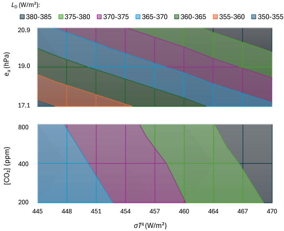
Figure 7.23 Changes in the downwelling LW radiation, L_D , as calculated by MODTRAN, due to changes in temperature (converted to blackbody radiation, \sigma T^4 ), and (upper) water vapour pressure ( e_a ) and (lower) carbon dioxide concentration ( [CO_2] ). The calculations were made for the tropical profile, no clouds and default other settings. For the upper graph it was assumed [CO_2] = 400 ppm and for the lower graph e_a = 19 hPa. Notice that the scale of the vertical axis is linear in the upper graph (with range \pm 10\% of the central value) and logarithmic in the lower graph (with range from half to twice the central value). (Source: Koutsoyiannis, 2024.)
