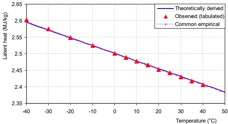
Figure 6.14 Comparison of latent heat of water as given by equation (6.199) and with standard tabulated data from List (1951), as well as with a common empirical equation (Shuttleworth, 1993), which is L/(\text{J kg}^{-1}) = 2.501 \times 10^6 - 2361 T/^\circ\text{C} . (Source: Koutsoyiannis, 2012.)
