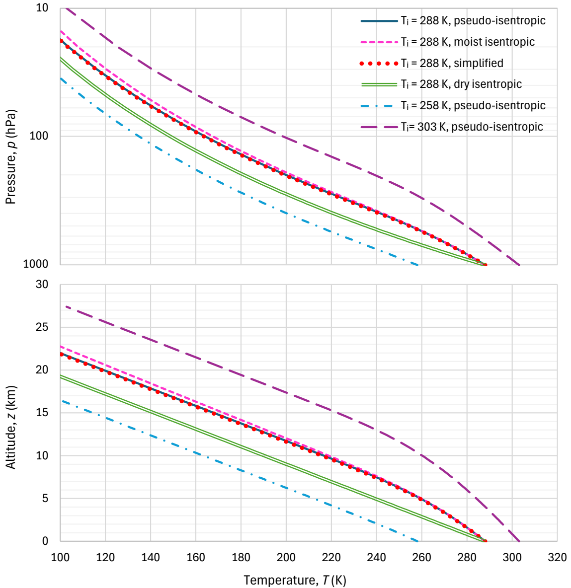
Figure 6.17 (upper) Illustration of isentropic changes as functions between total pressure p and temperature T that have the same total entropy per unit mass, for the indicated initial conditions defined as p_i = 1010 hPa, T_i as shown. (lower) Vertical temperature profiles derived from the isentropic curves of the upper panel, after translating pressure into altitude using the hydrostatic equation. For the calculations, the saturation vapour pressure was determined from equation (6.200) for temperatures higher than 0^\circ\text{C} = 273.15 K and (6.202) for lower temperatures.
