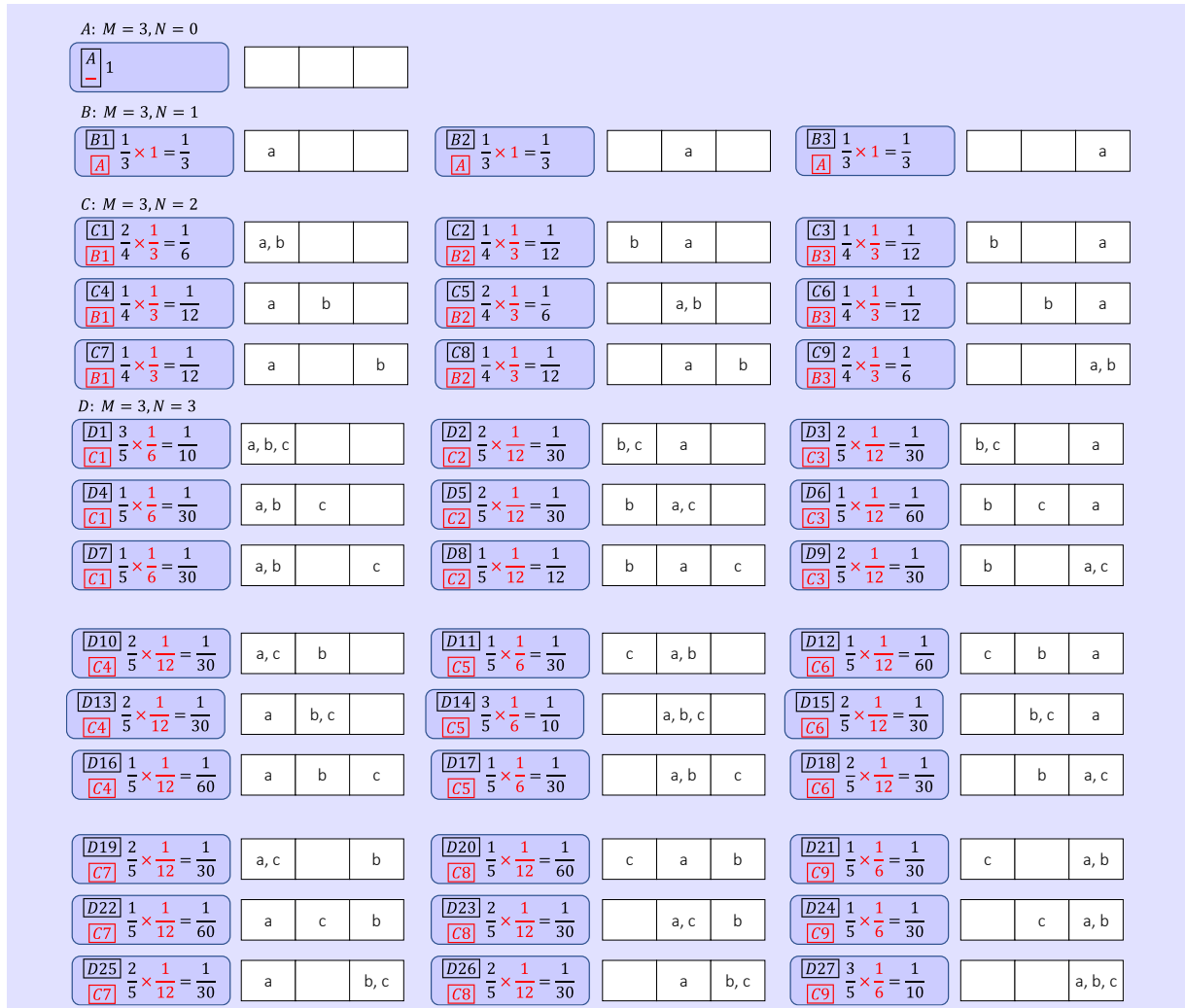
Figure 5.3 Illustration of calculating probabilities of all possible arrangements of placing N positively dependent particles (bosons), designated as a, b, c, into M = 3 boxes, where N is progressively increasing from 1 to 3. Each arrangement is assigned a particular label (B1, B2, etc.; upper left in each container of calculations) accompanied with the label of the predecessor arrangement (lower left in each container of calculations). In each calculation the first term is the conditional probability according to equation (5.16) and the second term is the probability that the condition holds (from the predecessor arrangement, i.e. the calculation is: conditional probability \times predecessor probability equals probability of this arrangement).
