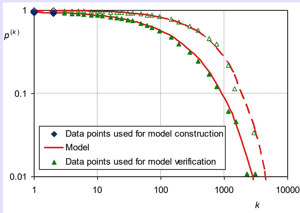
Figure 6.23 Probability dry p^{(k)} vs. scale k (in hours), as estimated from the Athens rainfall data set and predicted by a multiscale entropy maximization framework for the entire year (full triangles and full line) and the dry season (empty triangles and dashed line). (Source: Koutsoyiannis, 2006.)
