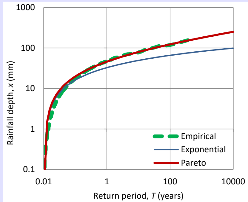
Figure 2.7 Rainfall depth vs. return period for Bologna based on 19 426 daily rainfall depths observed throughout the observation period of 206 years.
