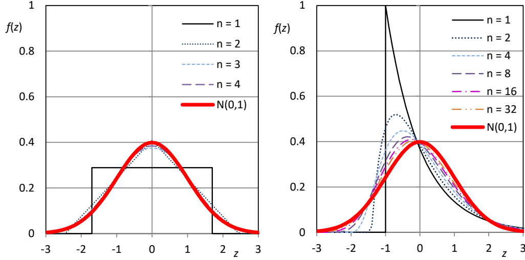
Figure 2.8 Convergence of the sum of independent identically distributed stochastic variables to the normal distribution (thick line). The thin continuous lines represent the probability density of the constituent variables \underline{x}_i , which have mean 0 and standard deviation 1. In the left panel the density is uniform on the interval (-\sqrt{3}, \sqrt{3}) with f(x) = \frac{1}{2\sqrt{3}} and in the right panel exponential, f(x) = e^{-x-1}, x \geq -1 (the parameters are chosen so as to have mean 0 and standard deviation 1). The dotted lines represent the densities of the sums \underline{z}_n := (\underline{x}_1 + \dots + \underline{x}_n)/\sqrt{n} for the values of n indicated in the legend. (The division of the sum by \sqrt{n} improves the presentation of the curves, as all \underline{z}_n have the same mean and variance, 0 and 1, respectively, and does not affect the essentials of the central limit theorem.) Equations (2.53) and (2.138) were used to produce the graph.
