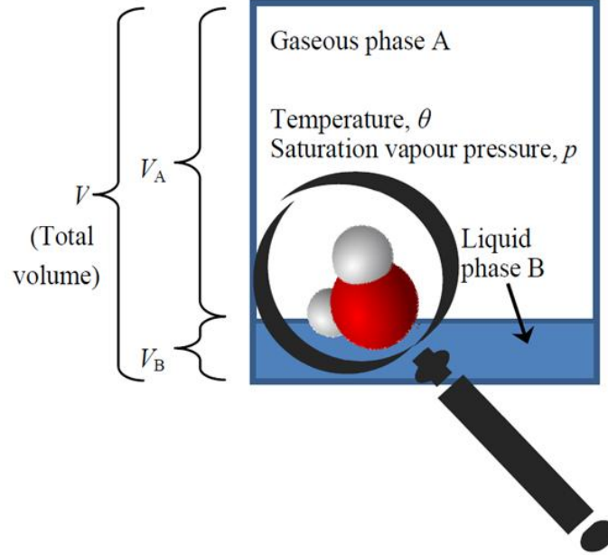
Figure 6.13 Explanatory sketch indicating the basic quantities involved in the equilibrium of water vapour with liquid water, zooming in on a single “shy” molecule which “tries to hide itself” by maximizing the combined uncertainty \varphi related to its phase (being either gaseous or liquid with probabilities P_A and P_B , respectively), position and kinetic state.
