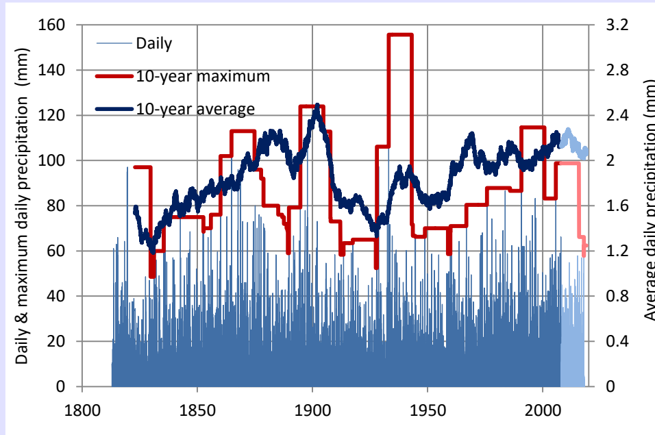
Figure 2.6 Plot of the time series of daily rainfall in Bologna, along with moving averages and moving maxima for a time window of 10 years (right-aligned, i.e., the value plotted at a specific year is the average or the maximum of the previous 10 years). The lines in darker colour represent the GHCN time series while those in lighter colour represent the newer data which are not included in the GHCN time series.
