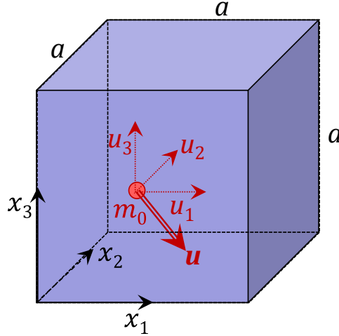
Figure 6.2 Explanation sketch for the collision of a molecule to the bottom face of a cube. The particle shown, located at coordinate x_3 (distance from the bottom face), will collide with the bottom face ( x_3 = 0 ) within time \delta t if x_3 \leq -u_3 \delta t . The other location and velocity coordinates do not play any role: for example, if x_1 and/or u_1 are large, a collision with the rightmost face of the cube may occur within \delta t , which however will result in horizontal reflection that will not alter the velocity coordinate u_3 .
