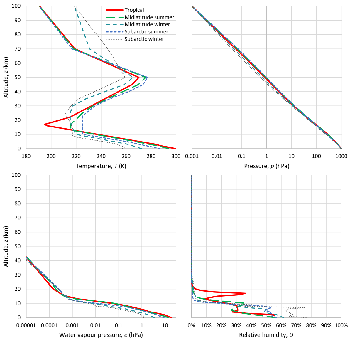
Figure 6.19 Vertical profiles of the indicated variables used in MODTRAN (Source: Koutsoyiannis, 2024).
