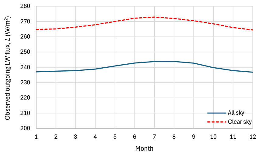
Figure 7.12 Monthly variation of outgoing LW radiation flux for 2024. The annual average is 240 and 268 W/m 2 for all sky and clear sky, respectively. Data from NASA's CERES site for Terra platform (Edition 4.2; https://ceres-tool.larc.nasa.gov/ord-tool/jsp/SSF1degEd42Selection.jsp ).
