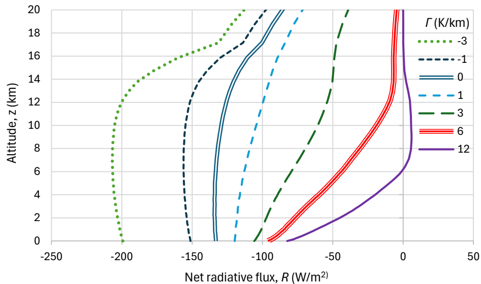
Figure 7.19 Vertical distribution of net radiation flux for the RRTM runs of Figure 7.17, for different lapse rates.
