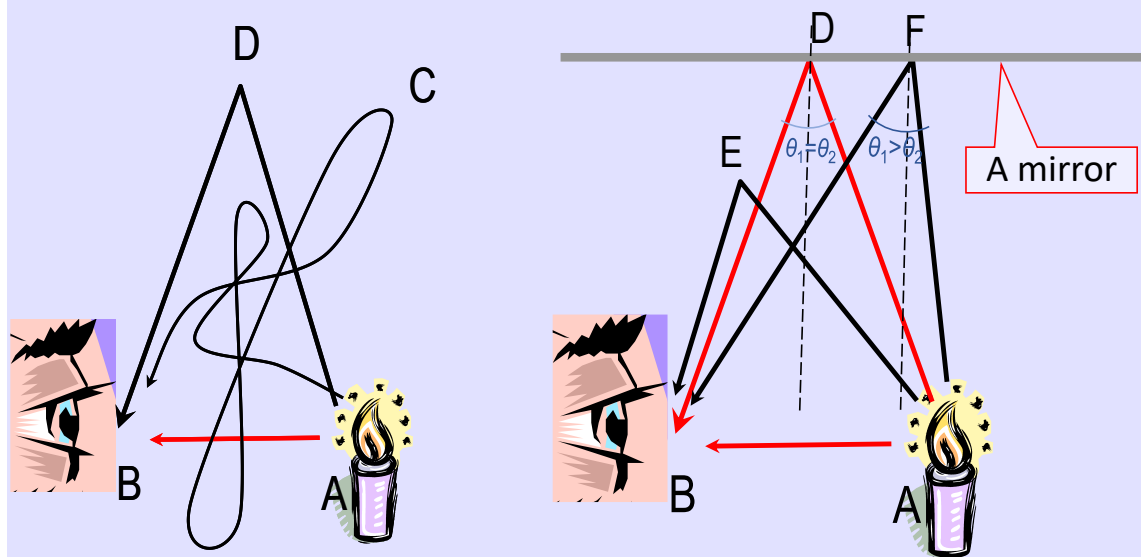
Figure 1.6 (left) The light from the candle A to an observer's eye B follows the simplest straight-line path AB (the red line) and not other more complex ones (e.g., the black lines ACB, ADB). (right) After putting a mirror at D, parallel to AB, the light follows the broken-line path ADB in addition to the straight-line path AB.
