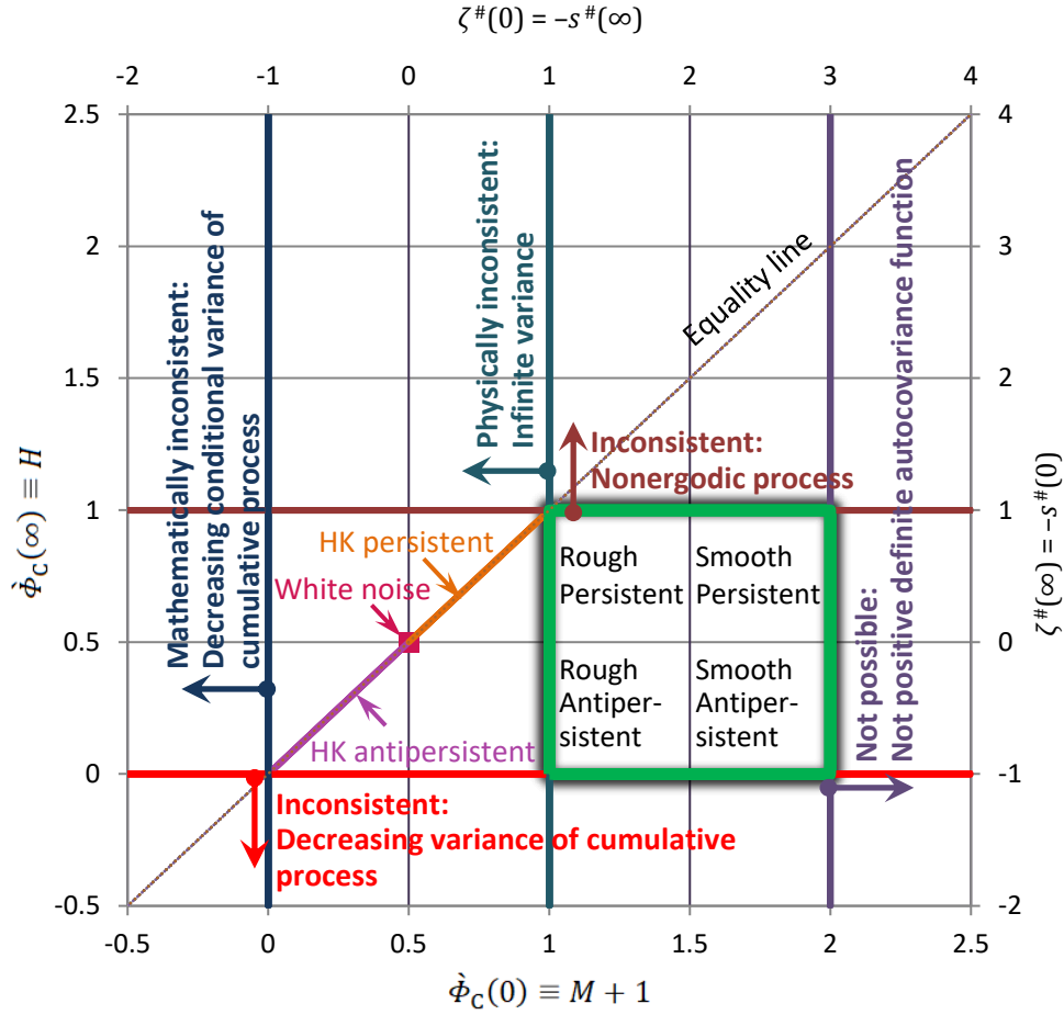
Figure 3.4 Bounds of asymptotic values of CEPLT, \hat{\phi}_C(0) and \hat{\phi}_C(\infty) , and corresponding bounds of the log-log slopes of power spectrum and climacospectrum. The “green square” represents the admissible region; note that s^\# can, by exception, take on values out of the square when \hat{\phi}_C(0) = 2 ( M = 1 ) or \hat{\phi}_C(\infty) = 0 ( H = 0 ). The reasons why a process out of the square would be impossible or inconsistent are also marked. The lines \hat{\phi}_C(0) = 3/2 ( M = 1/2 ) and \hat{\phi}_C(\infty) = 1/2 ( H = 1/2 ) define neutrality (which is represented by a Markov process) and support the classification of stochastic processes into the indicated four categories (smaller squares within the “green square”). (Source: Koutsoyiannis, 2017.)
