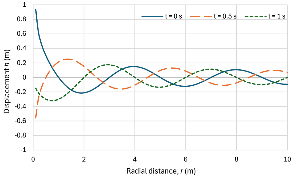
Figure 5.6 Displacement as a function of radial distance for water waves described by equation (5.37) for the indicated times. The assumed numerical constants are \varphi_0 = 0, c = 3 \text{ m/s} (corresponding to water depth of about 1 m), \lambda = 4 \text{ m}, a = 0.3 \text{ m}^{3/2} , so that T = c/\lambda = 0.75 \text{ s}, \nu = 1/T = 1.33 \text{ Hz} . The total energy per unit radius is 2\pi r e(r) = 2\pi r (1/2) \rho g a(r)^2 = \pi \rho g a^2 = \pi 1000 \text{ kg m}^{-3} 9.81 \text{ m s}^{-2} 0.3^2 \text{ m}^3 = 2773 \text{ kg m s}^{-2} or 2.77 \text{ kJ/m} .
