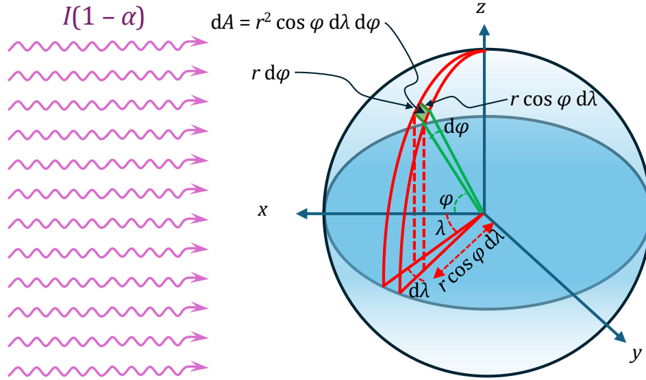
Figure 7.6 Schematic for the calculation of a planet's equilibrium temperature, with r , I and \alpha denoting the planet radius, the irradiance and the albedo, respectively.
