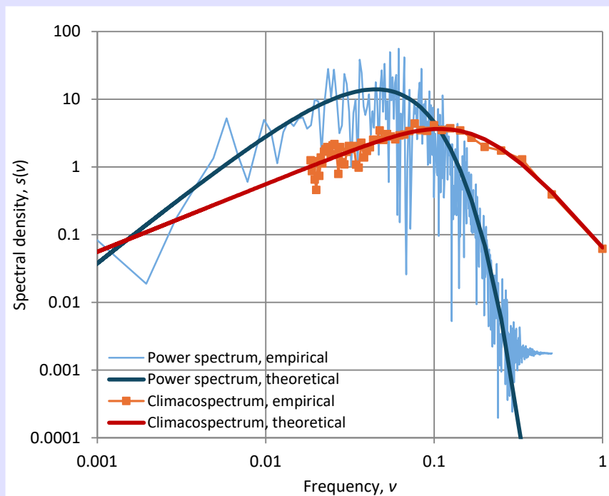
Figure 7.5 Empirical (estimated by the generated time series) and theoretical power spectrum (determined from the exact model) and climacospectrum (determined from equation (3.23)).
