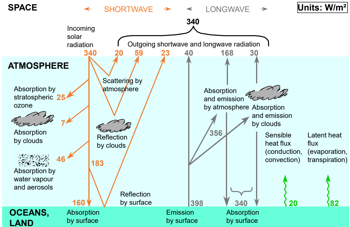
Figure 7.9 Schematic representation of the global mean energy budget of the Earth. The units are \text{W/m}^2 . The incoming solar radiation has been divided by 4, the ratio of Earth's area to its projection on a plane perpendicular to the Sun's rays. For the entire Earth's area ( 510.1 \times 10^6 \text{ km}^2 ) the incoming solar radiation and the outgoing total radiation equal 173.4 PW or 5470 ZJ/year. Only the latent heat which fuels the hydrological cycle is 1320 ZJ/year. For comparison, the total human primary energy consumption according to the most recent estimates, is 0.625 ZJ/year (2100 times smaller than the latent heat). The estimates are based on Ahrens (1993, pp. 38-41), Trenberth et al. (2009) and IPCC (2021; Figure 7.2), after adaptation. The emission of longwave radiation by Earth's surface was kept as in the last source but may be underestimated: for an average surface temperature of 288 K and emissivity 0.95, the emission would be 271 \text{ W/m}^2 if temperature were uniform, but this should be multiplied by the ratio (0.707/0.681)^4 following equation (7.57), which would result in a value 8% higher than shown in the figure.
