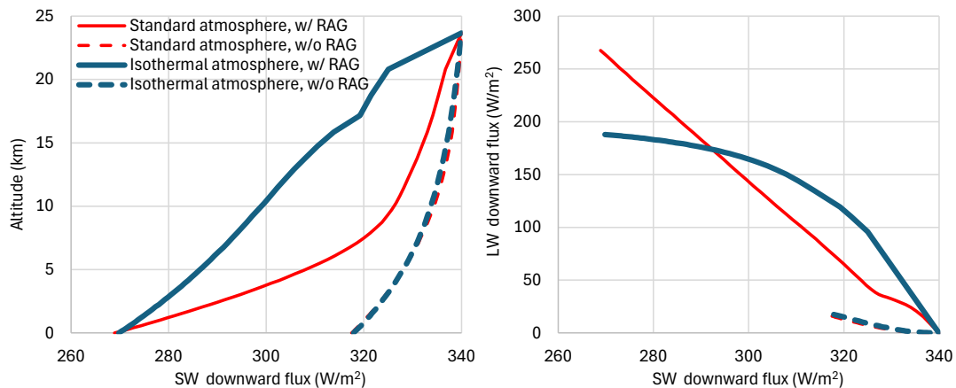
Figure 7.22 (left) SW downward energy flux as a function of altitude for the indicated cases (standard or isothermal atmosphere, with or without RAGs and without clouds); (right) . LW downward energy flux as a function of SW downward energy flux for the same cases. The values plotted were calculated by RRTM with default values of the related parameters. (Reproduced from Koutsoyiannis and Tsakalias, 2025; Appendix SA.)
