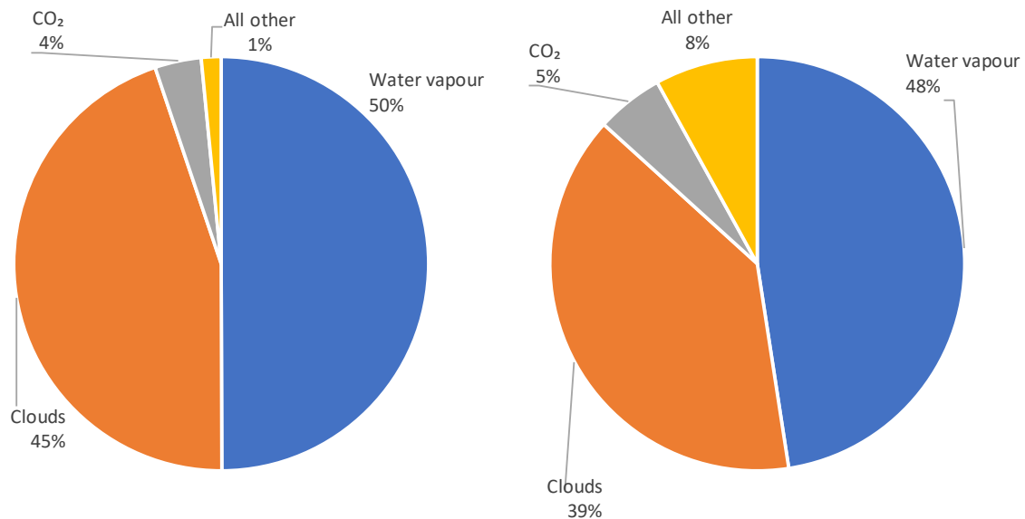
Figure 7.25 Contribution of the ARE drivers to the LW radiation fluxes, ( left ) downwelling and ( right ) outgoing. (Source: Koutsoyiannis, 2024.)
